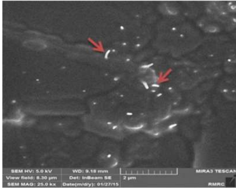
Figure 7. MWCNTs pull out in the matrix.
