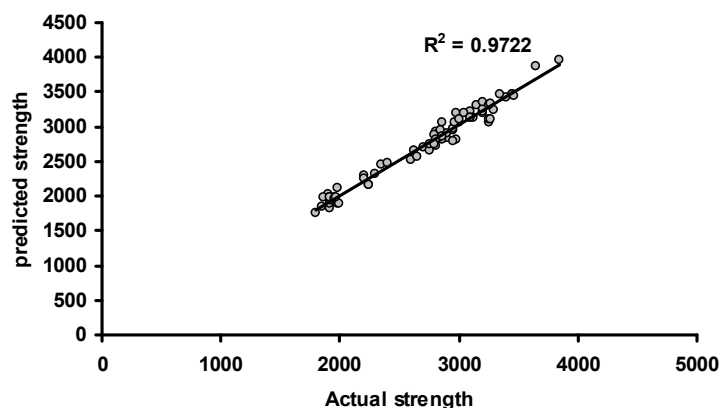
Figure 5- Line of best fit for predicted strength and the actual strength of carbon fibers by back propagation neural network model for training testes.
