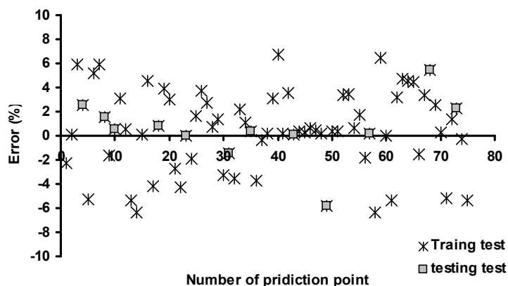
Figure 4- Comparison of % error of predicted results using back propagation neural network model for strength of carbon fibers.
