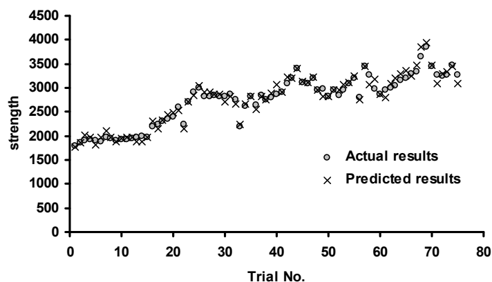
Figure 3- Comparison of predicted and actual results in predicting strength of carbon fibers while training using back propagation neural network model.
