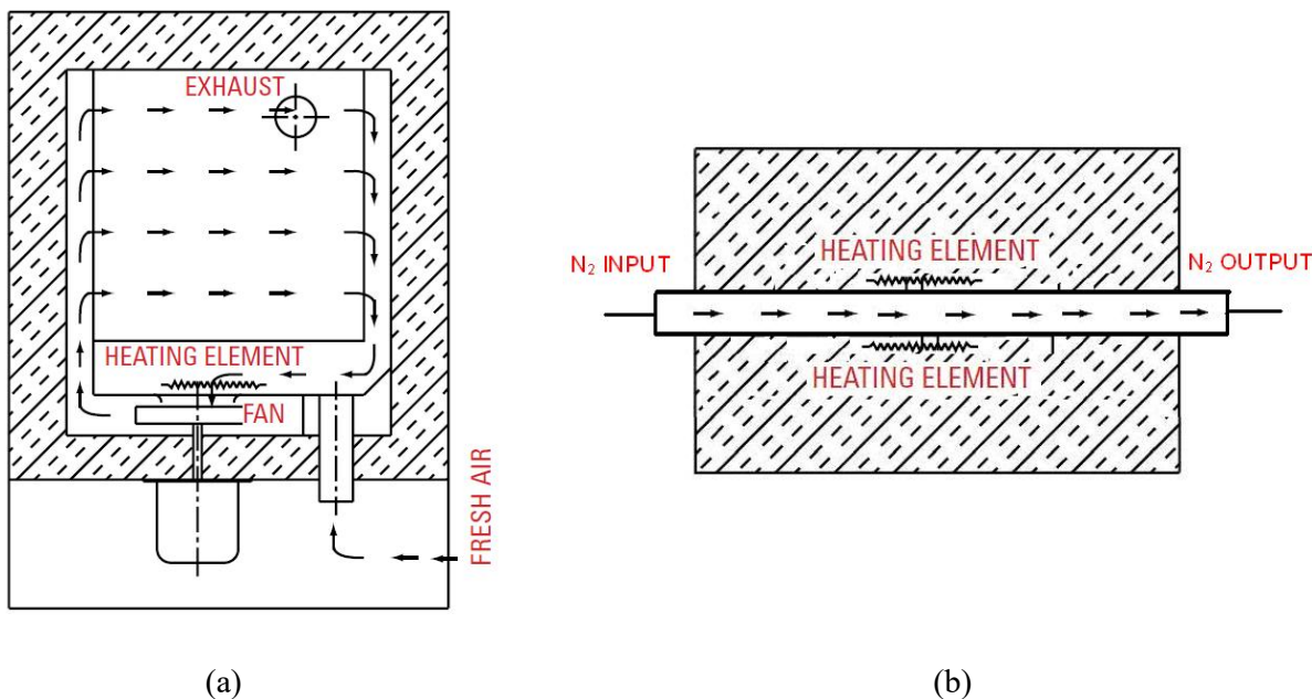
Figure 1- The schematics of; (a) stabilization furnace and (b) carbonization furnace.
