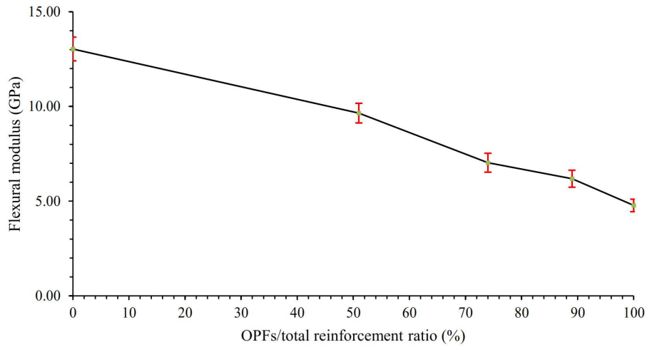
Figure 10. Flexural modulus of hybrid glass fibers- OPFs composites.
