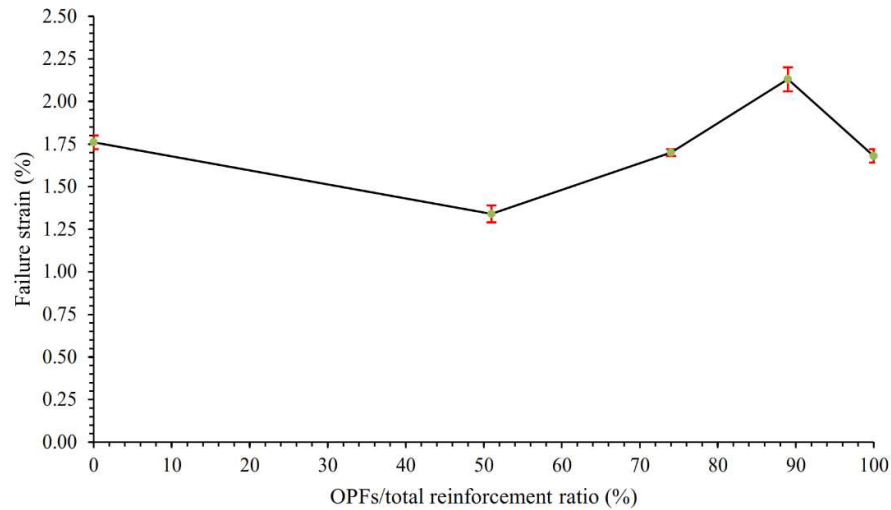
Figure 8. Failure strain of hybrid glass fibers- OPFs composites.
