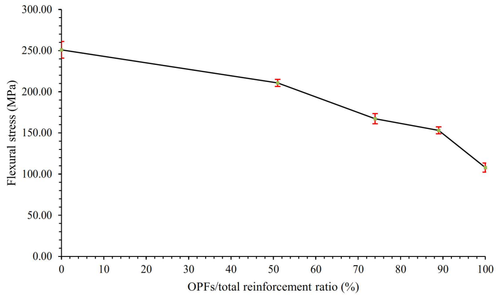
Figure 9. Flexural stress of hybrid glass fibers- OPFs composites.
