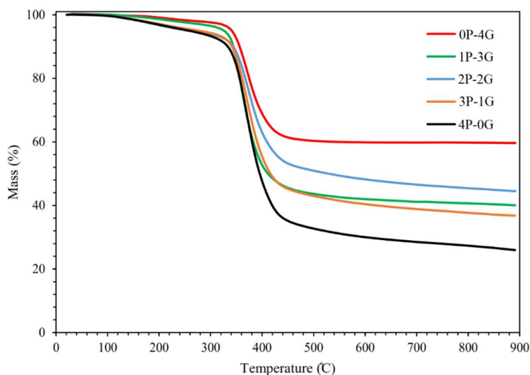
Figure 2. TG curves of hybrid glass fibers- OPFs composites.
