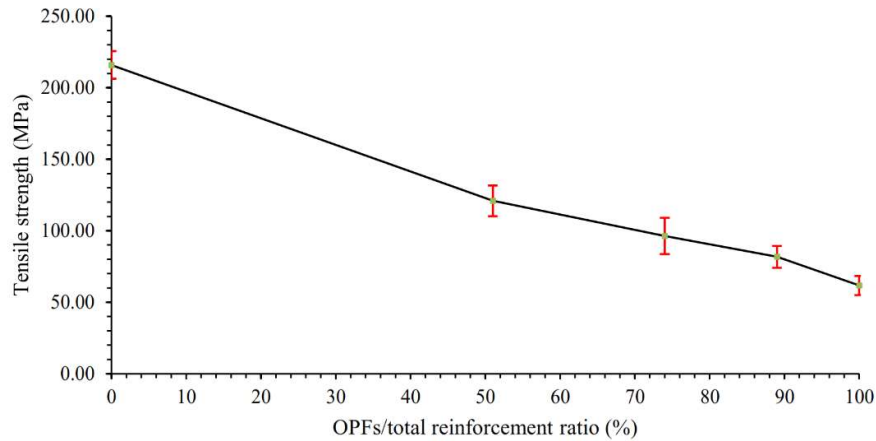
Figure 6. Tensile strength of hybrid glass fibers- OPFs composites.
