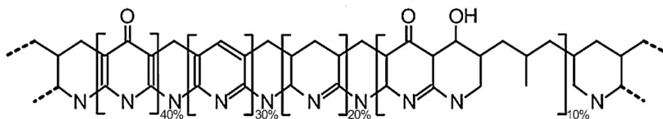
Figure 5. Chemical structure of stabilized PAN [8].
