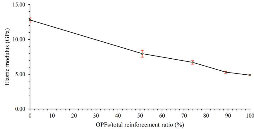
Figure 7. Elastic modulus of hybrid glass fibers- OPFs composites.
