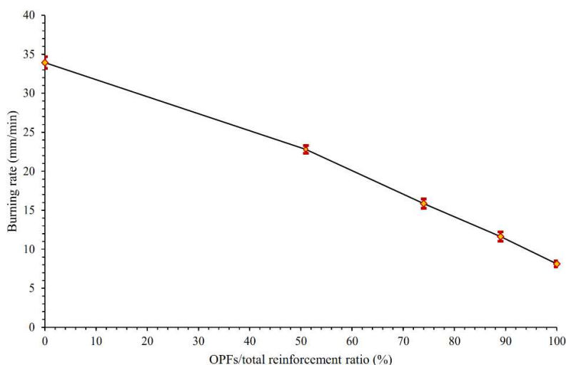
Figure 4. Burning rate of hybrid glass fibers- OPFs composites.
