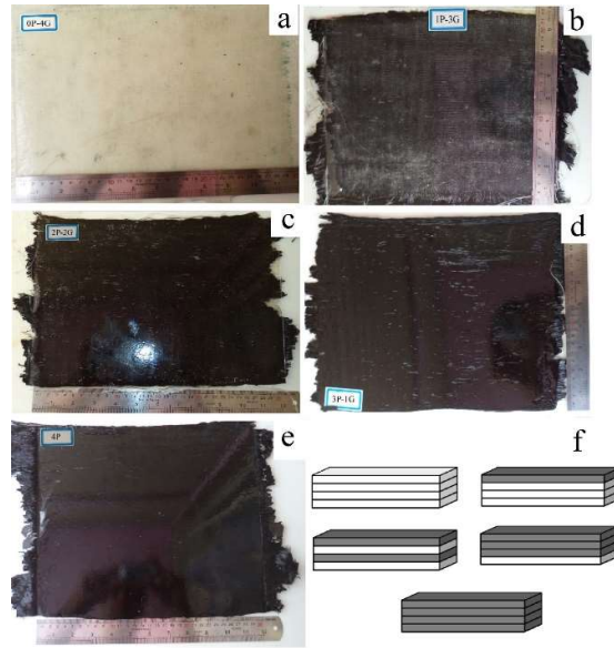
Figure 1. Fabricated hybrid composites; a: 0P-4G, b: 1P-3G, c: 2P-2G, d: 3P-1G, e: 4P-0G, f: Different stacking sequences (black layer: OPFs, white layer: glass fibers).
