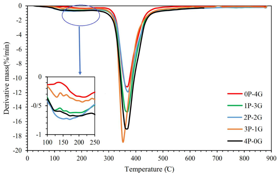
Figure 3. DTG curves of hybrid glass fibers- OPFs composites.
