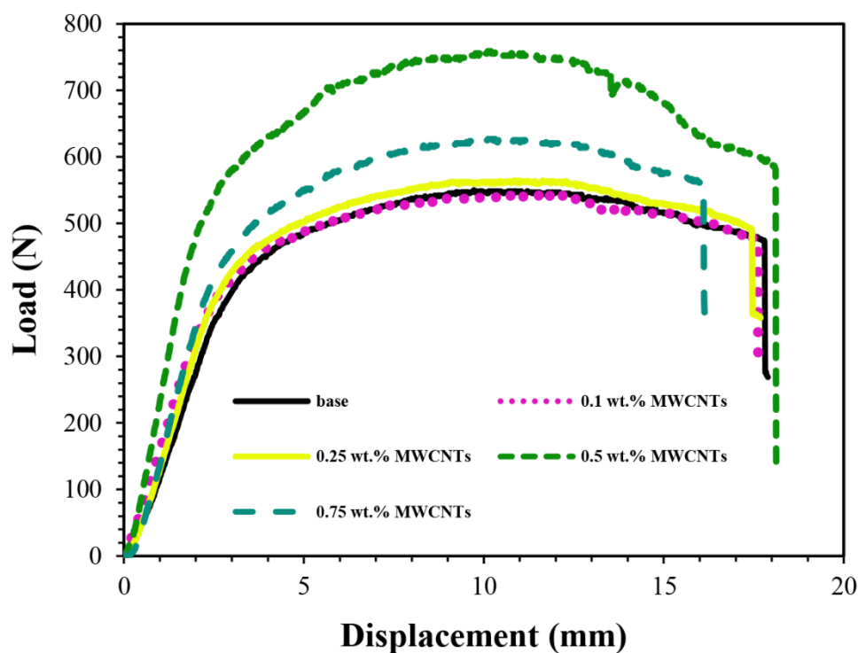
Fig. 2. The load-displacement curves obtained from flexural testing of basalt fibers/ epoxy/ aluminum 2024 laminates with different content of MWCNTs.
