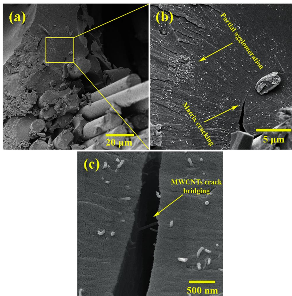
Fig. 7. FESEM images of fracture surface of basalt fibers/ epoxy composite containing 0.5 wt.% MWCNTs at magnifications of (a) 2000X, (b) 10000X and (c) 75000X.
