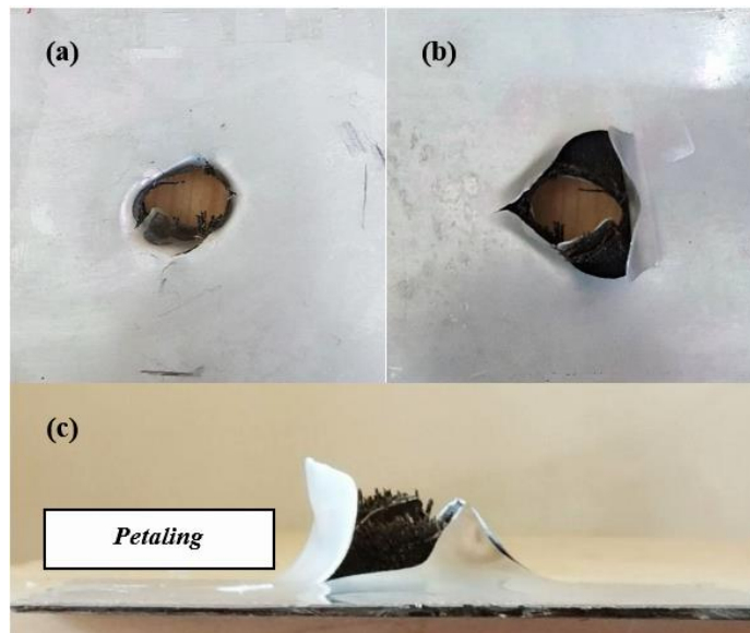
Fig. 9. Damage mode of FMLs impacted by conical projectile (a) front face, (b) back face and (c) cross views.
