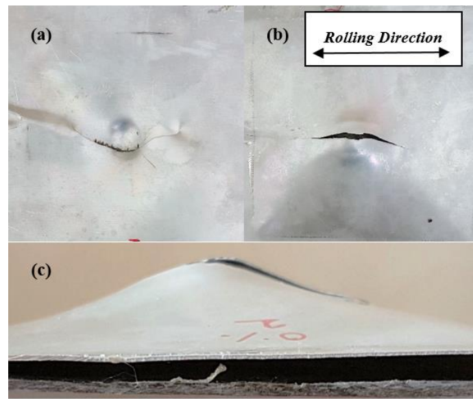
Fig. 8. Damage mode of FMLs impacted by hemispherical projectile (a) front face, (b) back face and (c) cross views.
