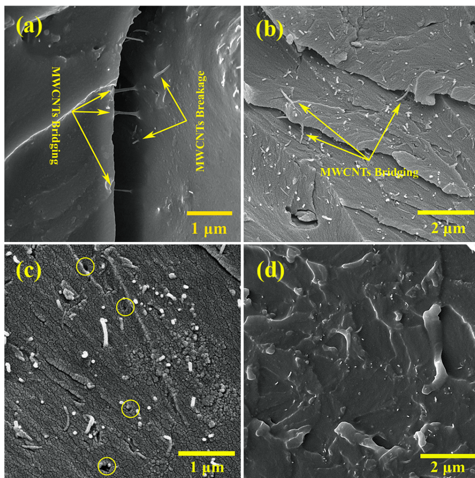
Fig. 6. The FESEM images of strengthening mechanisms of basalt fibers/epoxy composite containing 0.5 wt.% MWCNTs (a) MWCNTs-crack bridging, (b) MWCNTs-pull-out and bridging, (c) plastic void growth and (d) rough fracture surface.
