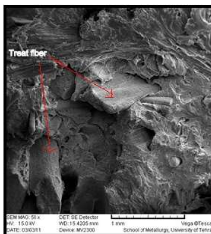
Figure 9. SEM micrographs of fracture surface of PP/EPDM with Treated fibers.
