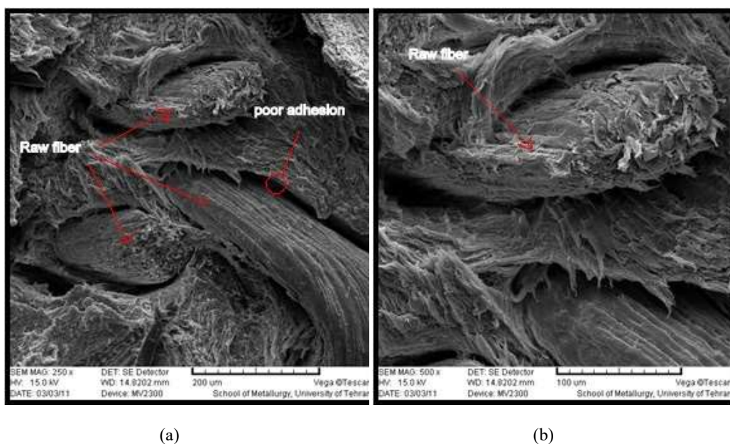
Figure 8. SEM micrographs of fracture surface of PP/EPDM with raw fibers.
