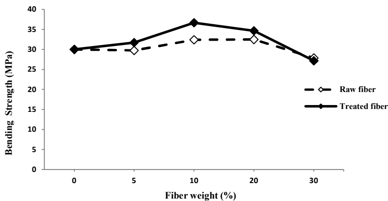
Figure 7. Variation of bending strength at different fiber weight fractions.
