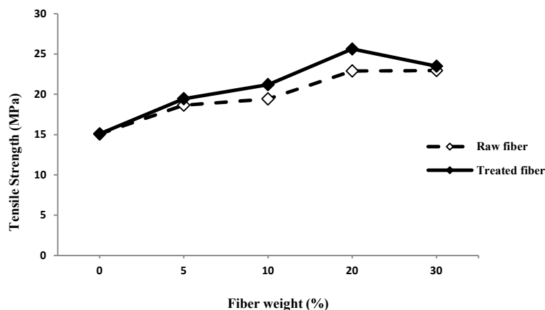
Figure 6. Variation of tensile strength at different fiber weight fractions.
