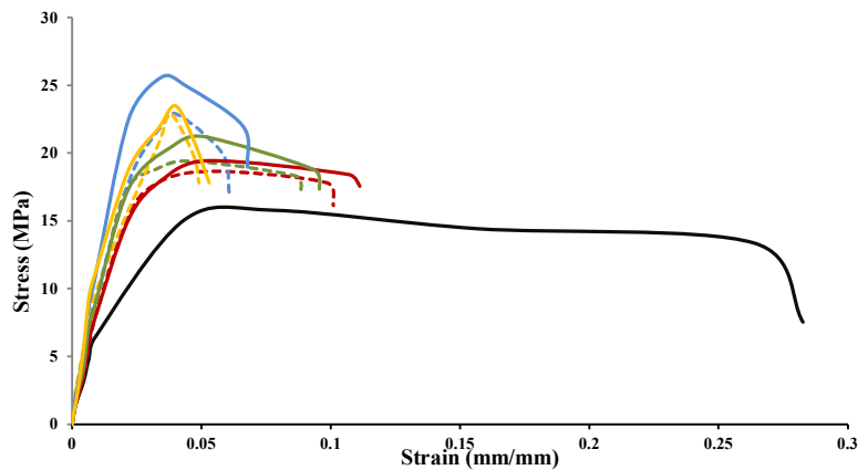
Figure 5. Stress-strain curves for PP/EPDM/DPF.
