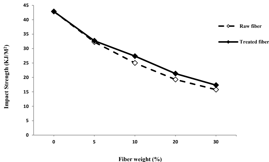
Figure 4. Variation of impact strength at different fiber weight fractions.
